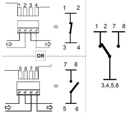
CONNECTION DETAILS
